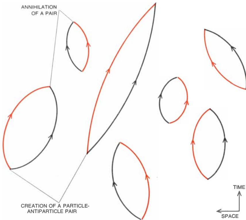
“EMPTY” SPACE-TIME is full of “virtual” pairs of particles ( black ) and antiparticles ( color ). Members of a pair come into existence simultaneously at a point in space-time, move apart and come together again, annihilating each other. They are called virtual because unlike “real” particles they cannot be detected directly. Their indirect effects can nonetheless be measured.
