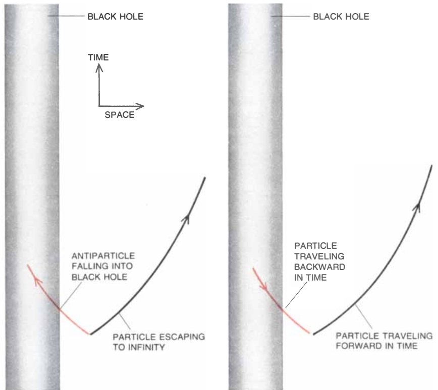
ALTERNATIVE INTERPRETATIONS can explain the emission of particles by a black hole. One explanation ( left ) invokes the formation of a virtual particle-antiparticle pair, one member of which is trapped by the black hole as the other escapes. In another explanation ( right ) one can regard an antiparticle falling into a black hole as being a normal particle that is traveling backward in time out of the black hole. Once outside it is scattered by the gravitational field and converted into a particle traveling forward in time, which escapes to infinity.
