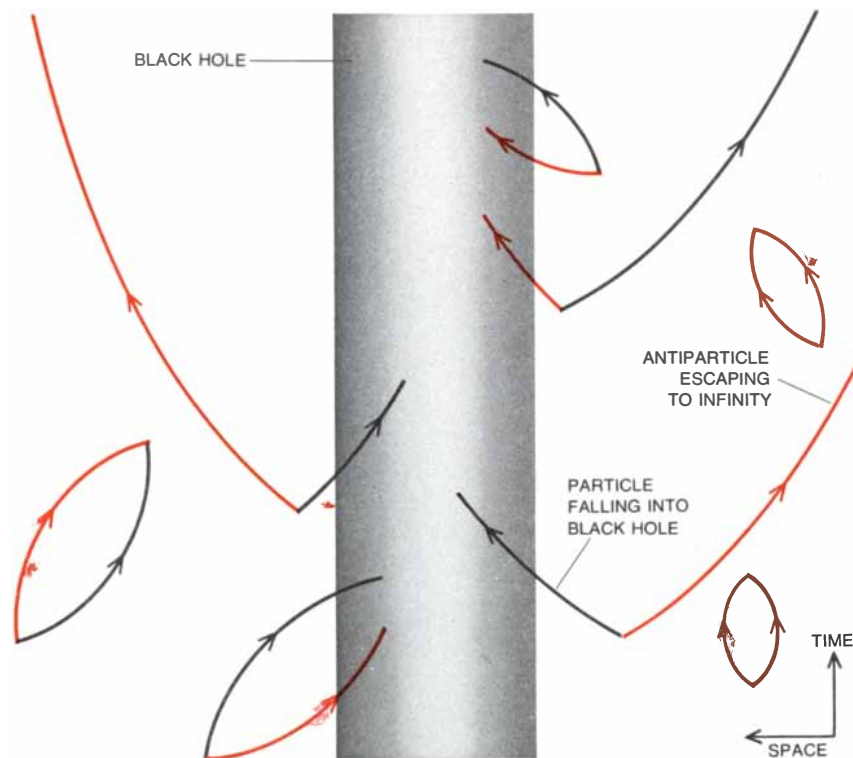
IN THE NEIGHBORHOOD OF A BLACK HOLE one member of a particle-antiparticle pair may fall into the black hole, leaving the other member of the pair without a partner with which to annihilate. If surviving member of pair does not follow its partner into black hole, it may escape to infinity. Thus black hole will appear to be emitting particles and antiparticles.
